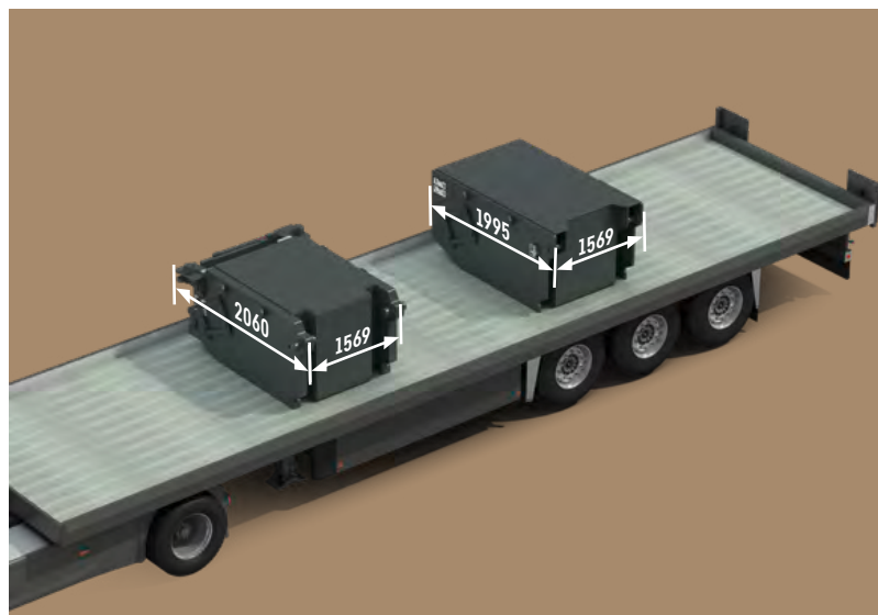
Zentralballast Center counterweight Contrepoids de base Zavorra centrale Contrapeso central Центральный балласт
