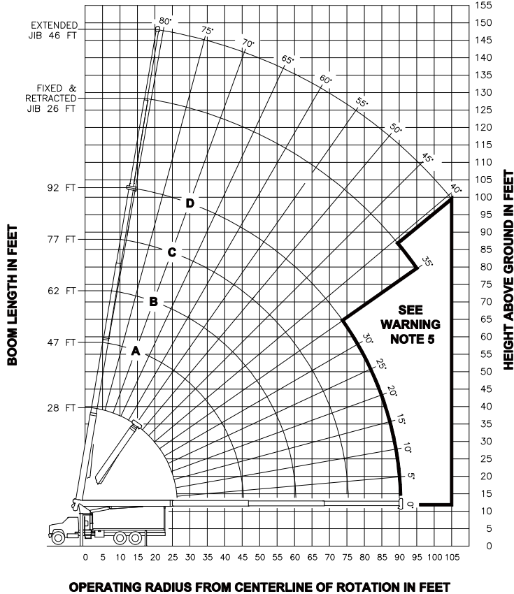
RANGE DIAGRAM
