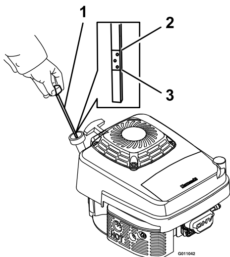
Figure 17 Kawasaki Engine
