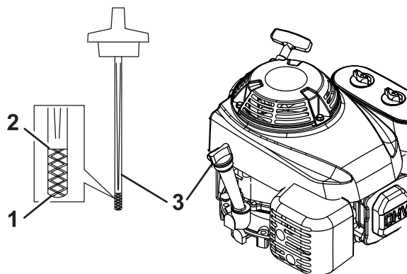
Figure 16 Honda Engine
