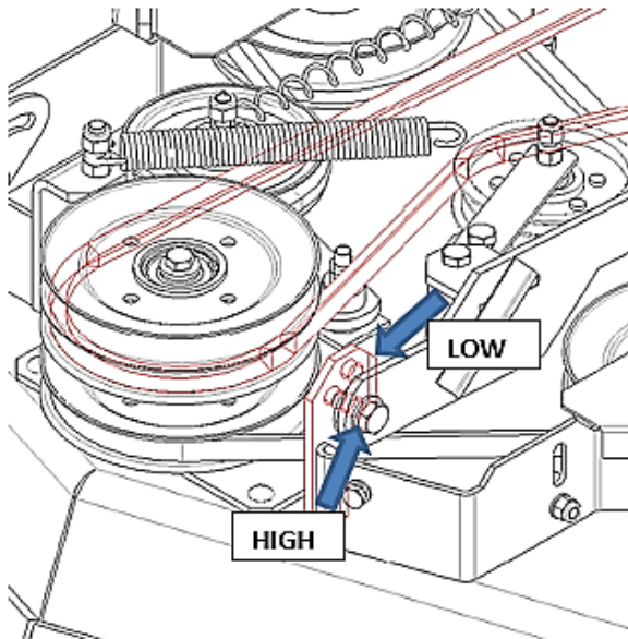
Belt and Floating Idler Bar shown in high range
