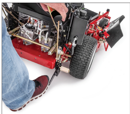
Walk Behind | Remote Discharge Control Float Deck Only
